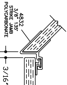
135° POLYCARBONATE STRIKE
