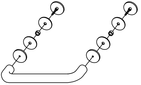
EPH-XXX-04803 TUBULAR SINGLE MOUNT HANDLE
