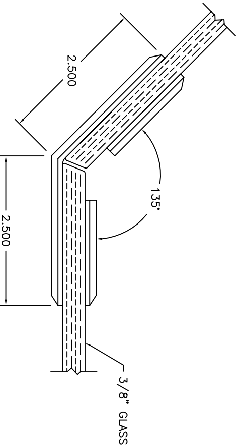
TOP VIEW OF GLASS TO GLASS CLIP FULL SIZE
