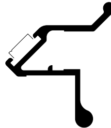
67287 Handle Rail w/V-253 Magnet
