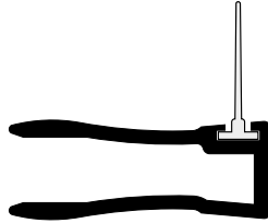
SC-540 62673 840 Pocket Rail with V-207 Vinyl
